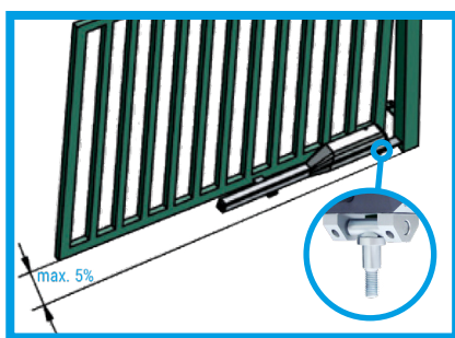
Swivelling connection for rising terrain
